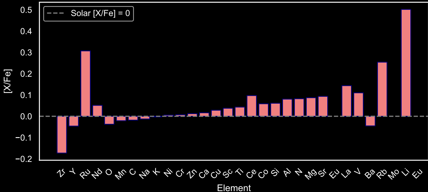
Abundance Pattern for GALAH Main Sequence Stars: Star Field [51] (N=48)
