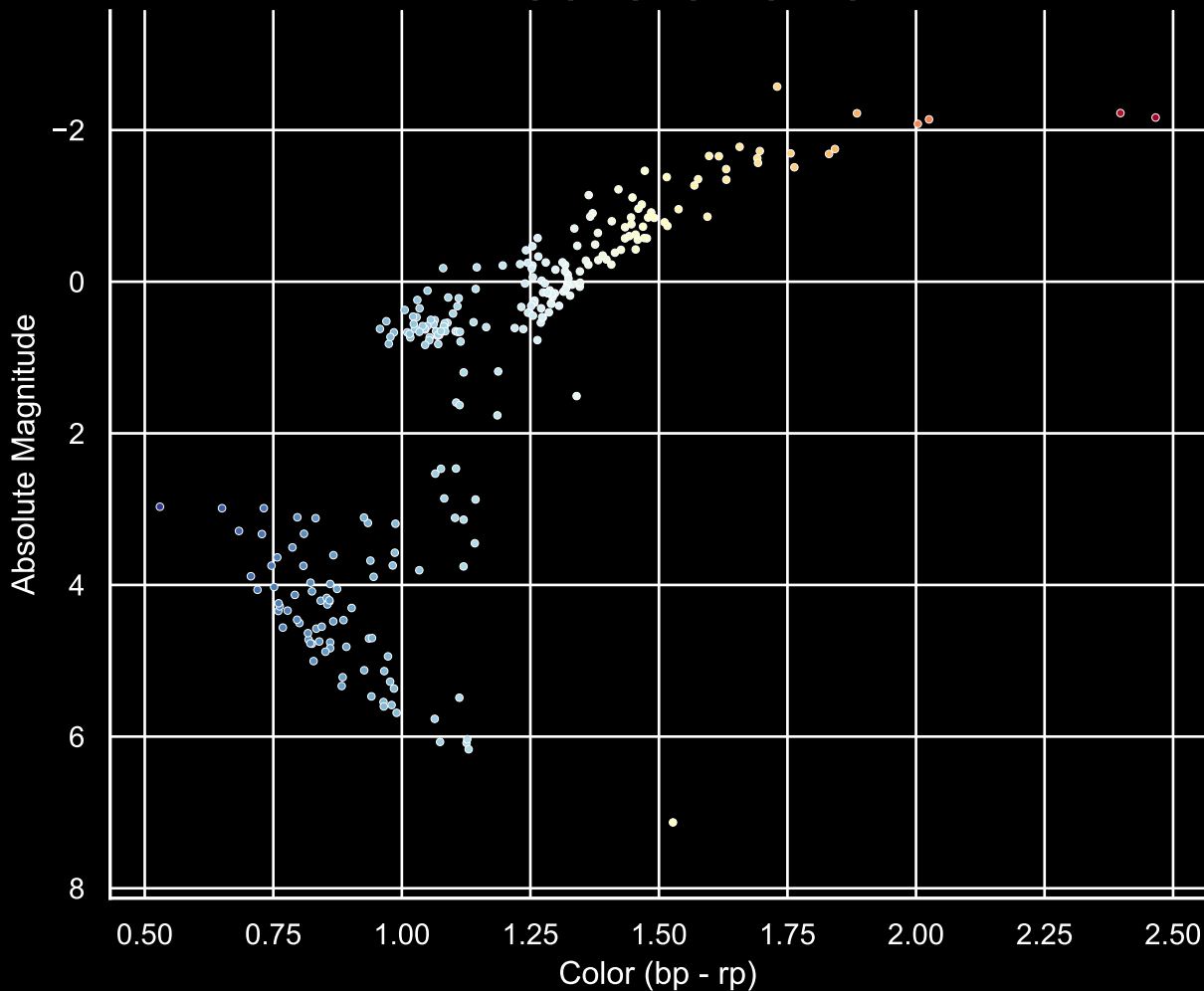
GALAH Hertzprung-Russel Diagram Field [51] Ra [6.28] Dec [-72.03]
