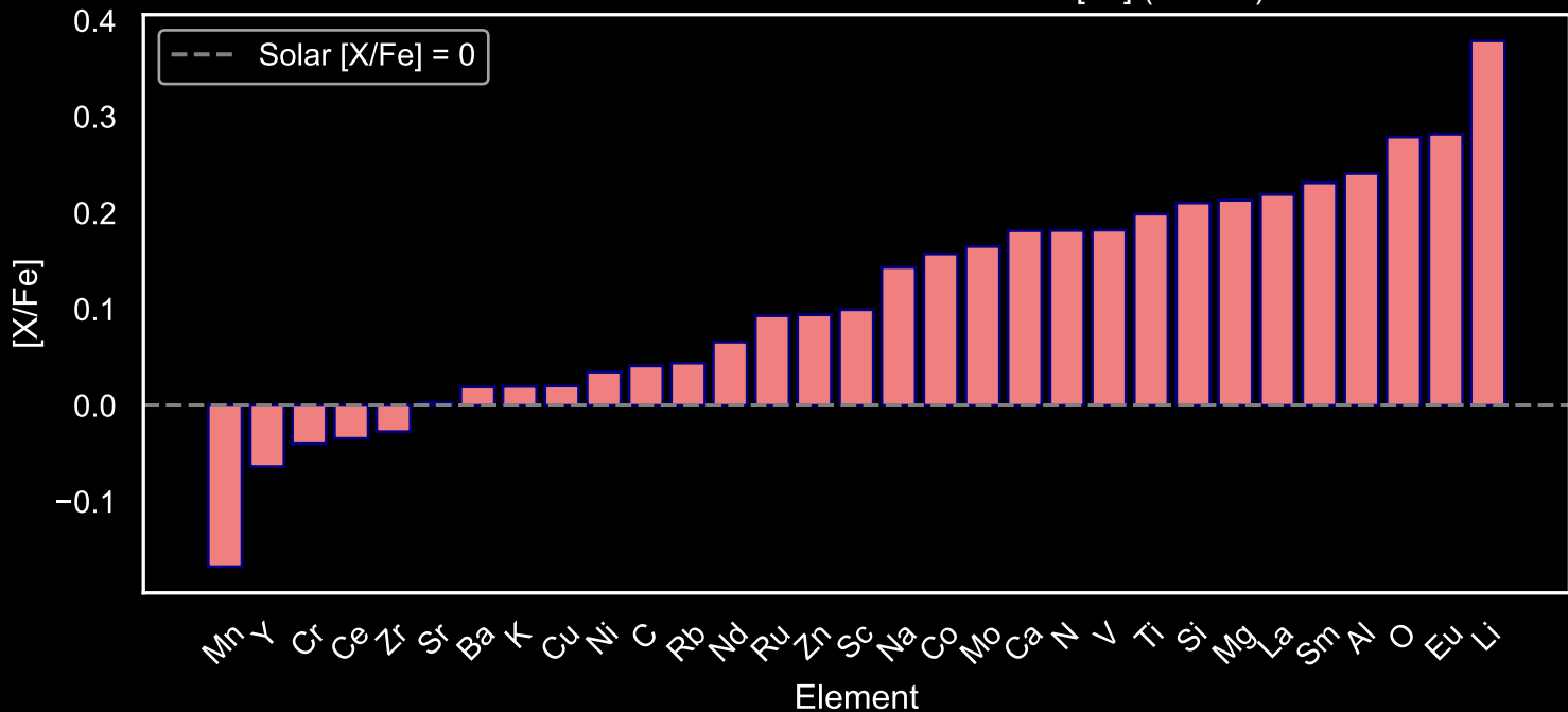
Abundance Pattern for GALAH Star Field [51] (N=260)
