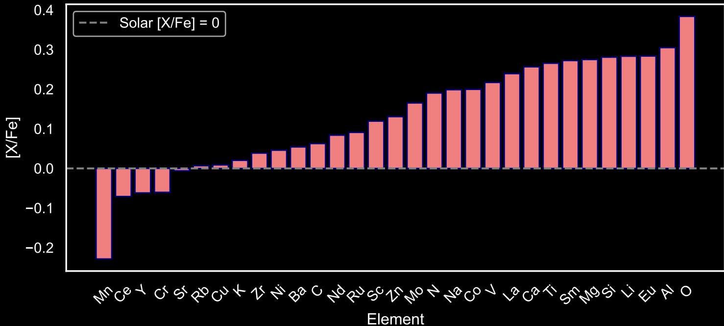
Abundance Pattern for GALAH Red Giants: Star Field [51] (N=180)
